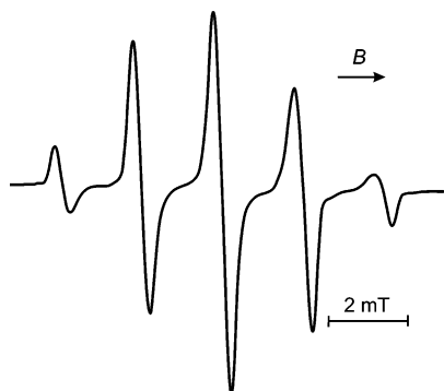
Figure 1. ESR spectrum of ionized dicyclopropylidenemethane ( 2 ) in a \text{CFCl}_3 matrix at 150 K.
