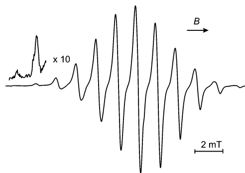
Figure 2. ESR spectrum of ionized octamethyldicyclopropylidenemethane ( 2-Me 8 ) in a \text{CFCl}_3 matrix at 140 K.
