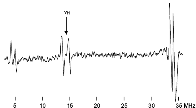
Figure 3. ^1\text{H} -ENDOR spectrum of ionized octamethyldicyclopropylidenemethane ( 2-Me 8 ) in a \text{CFCl}_3 matrix at 140 K.
